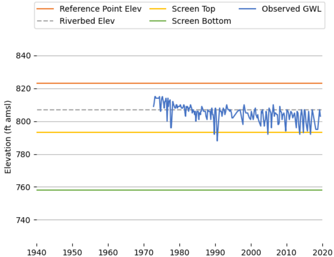
Figure K-27 Observed Groundwater Level (05N23W33B03S).
