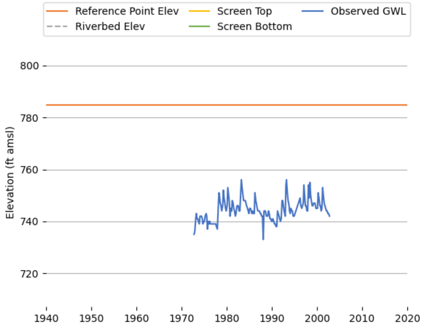
Figure K-13 Observed Groundwater Level (04N23W11D01S).
