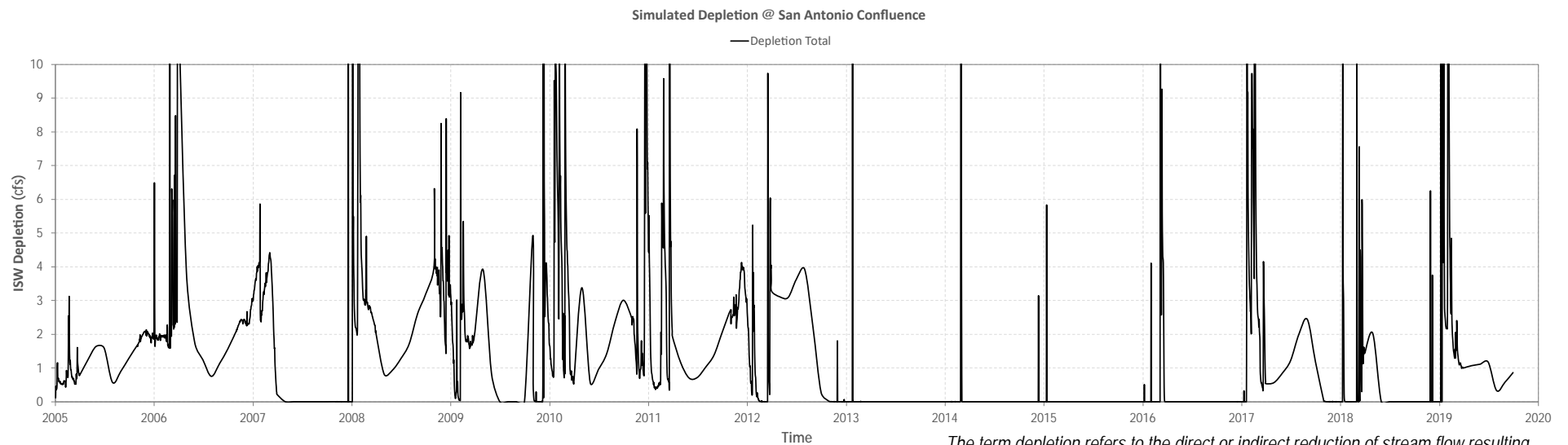
Figure N-07 Streamflow Depletion (San Antonio Confluence).
