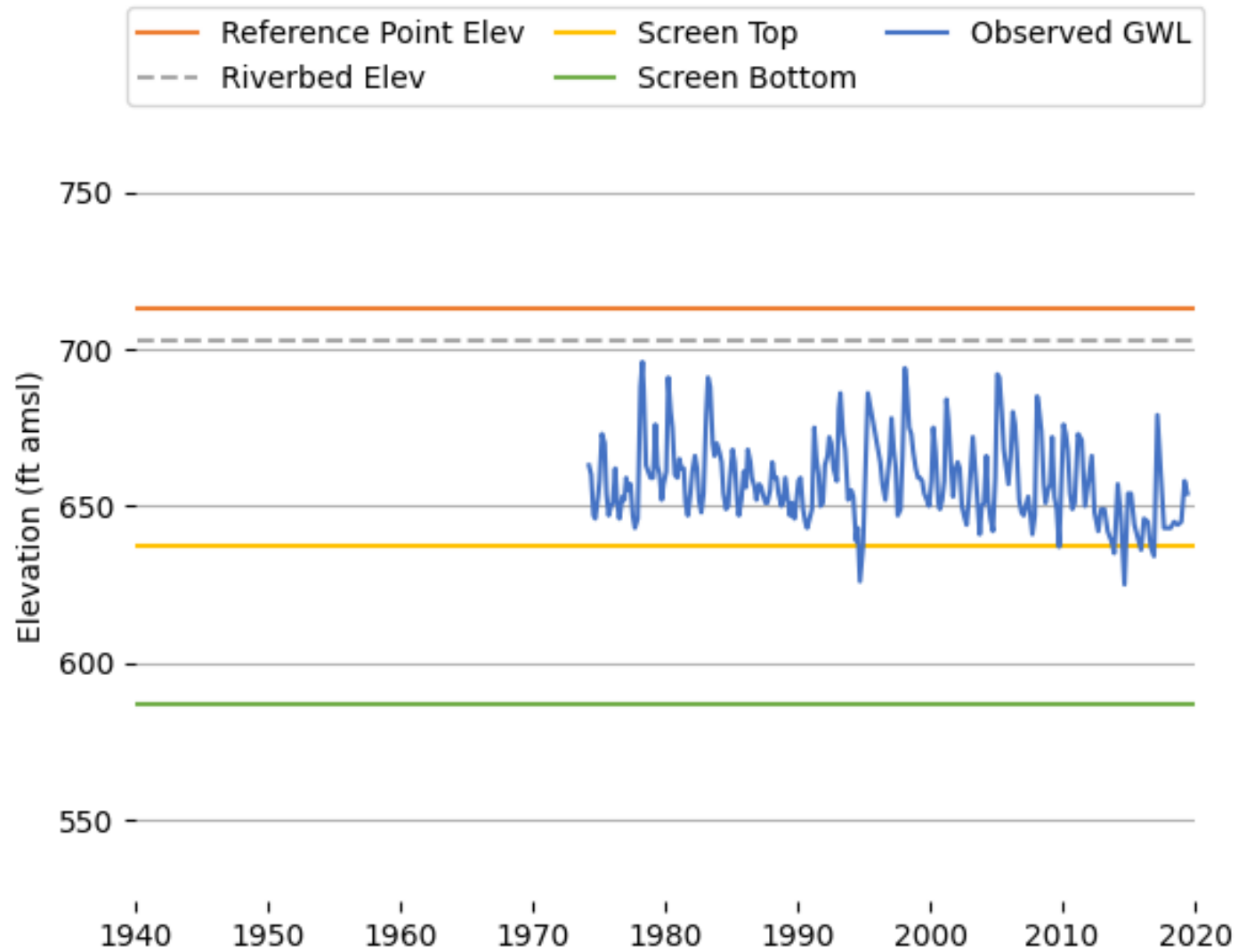
Figure K-10 Observed Groundwater Level (04N23W04J01S).
