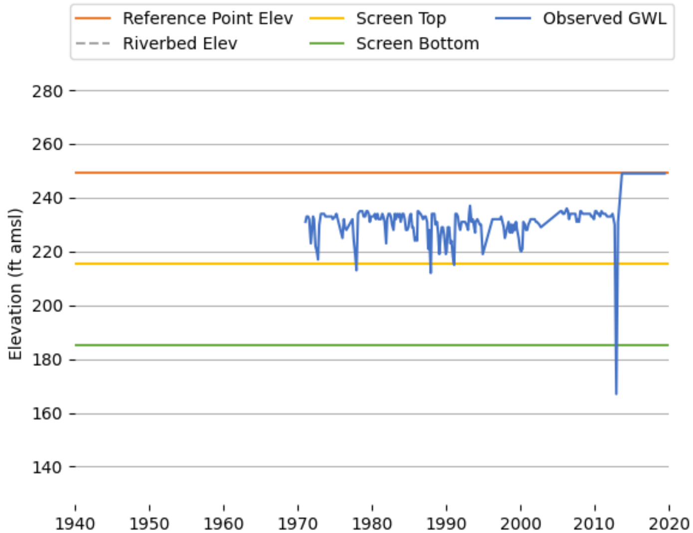
Figure K-05 Observed Groundwater Level (03N23W08B02S).
