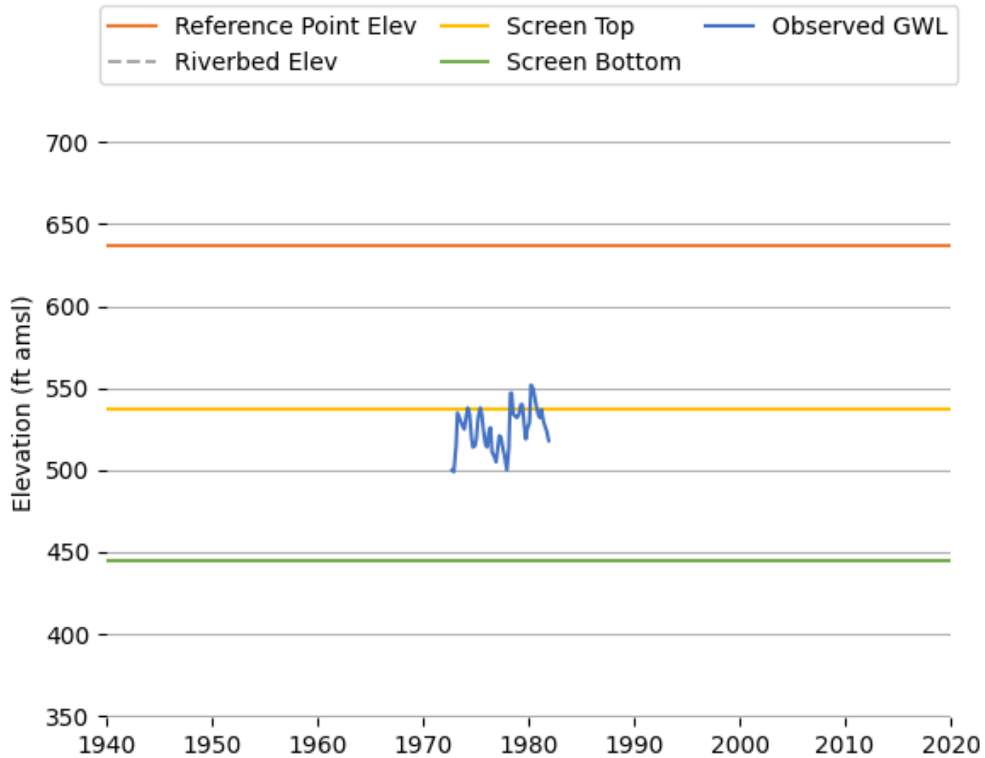
Figure K-16 Observed Groundwater Level (04N23W15D01S).
