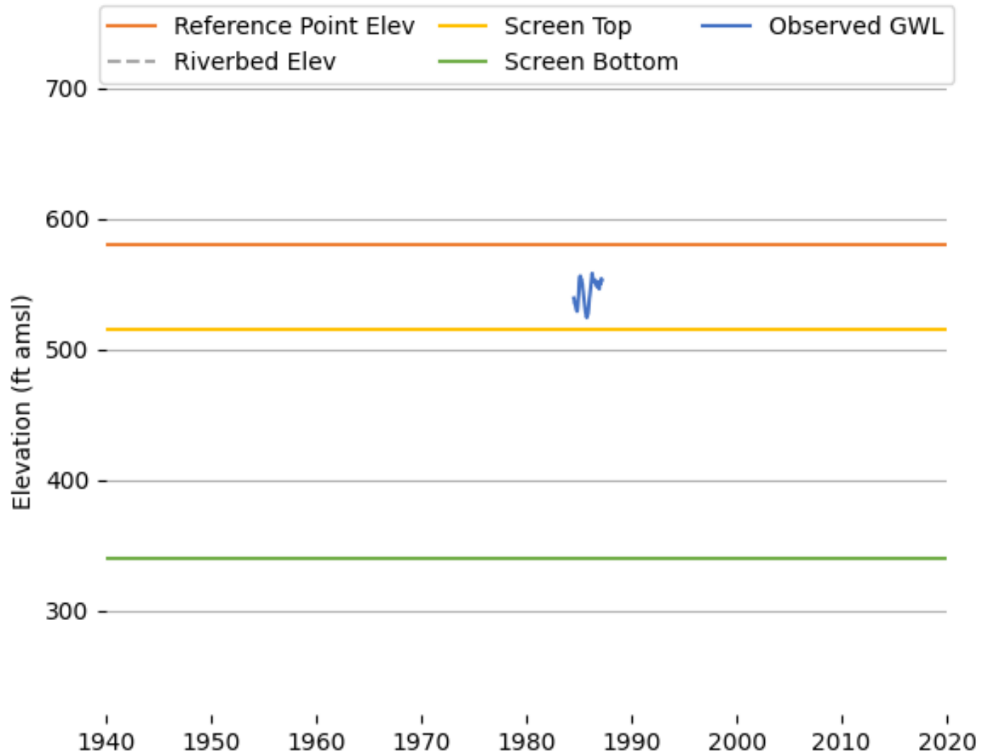
Figure K-20 Observed Groundwater Level (04N23W16C07S).
