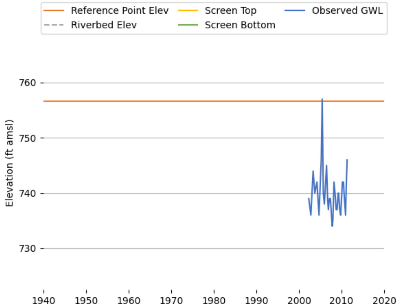
Figure K-30 Observed Groundwater Level (T0611100412_MW-2).
