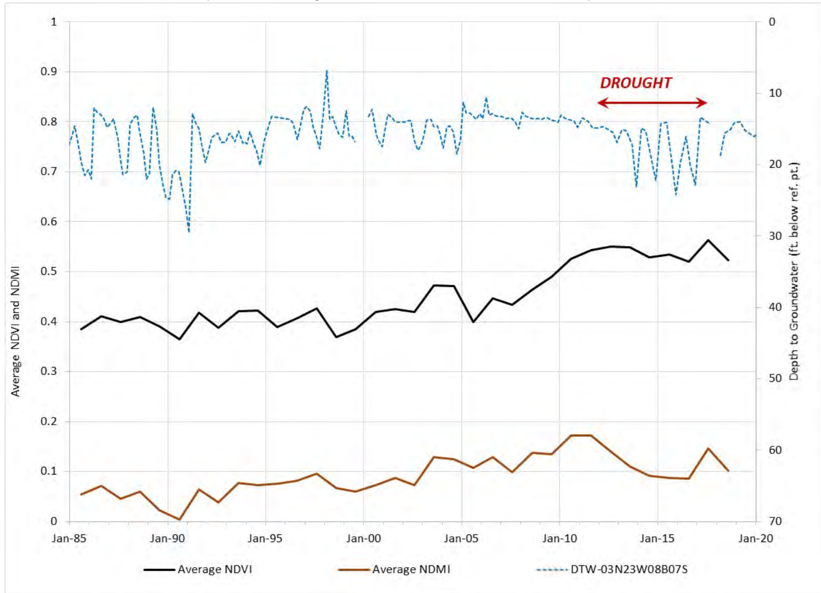
Figure 12 Groundwater Level Compared to Average NDVI and NDMI for the Foster Park Riparian GDE Unit (1985 to 2018)
