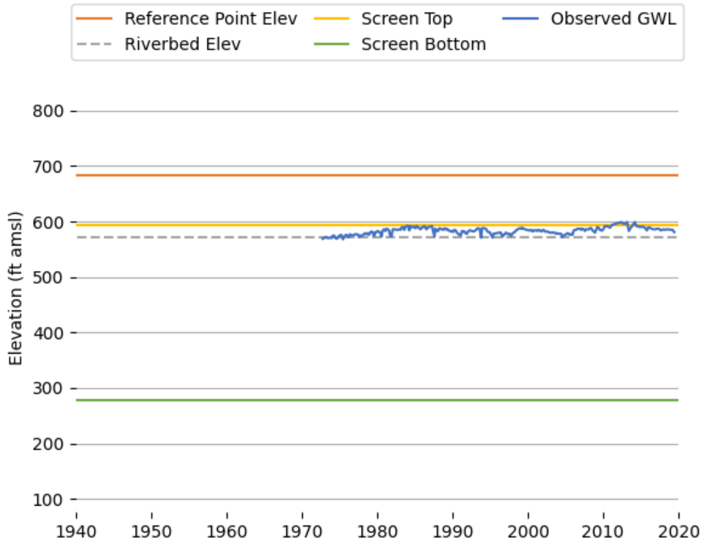
Figure K-14 Observed Groundwater Level (04N23W15A02S).
