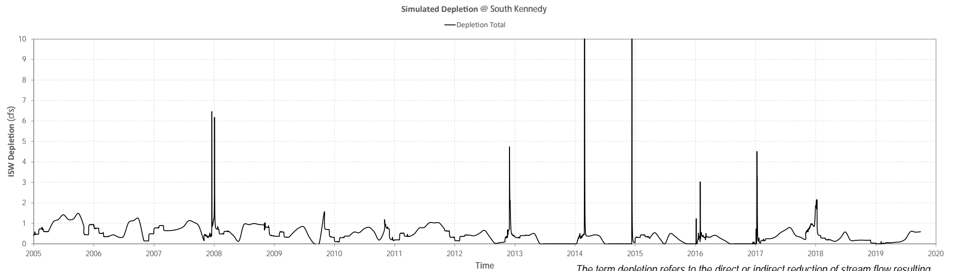
Figure N-02 Streamflow Depletion (South Kennedy).
