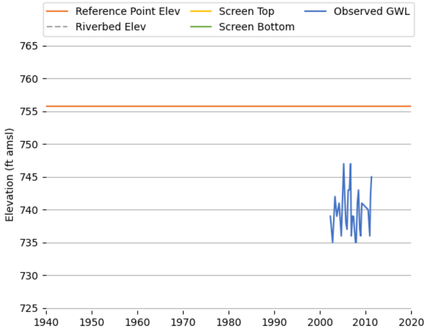
Figure K-34 Observed Groundwater Level (T0611100412_MW-6).
