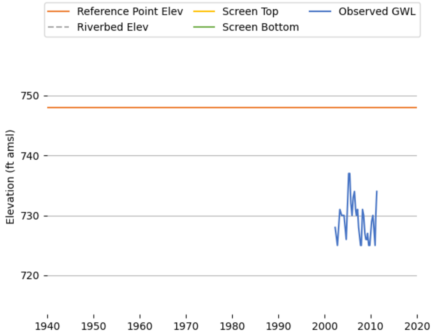
Figure K-49 Observed Groundwater Level (T0611100412_MW-21).
