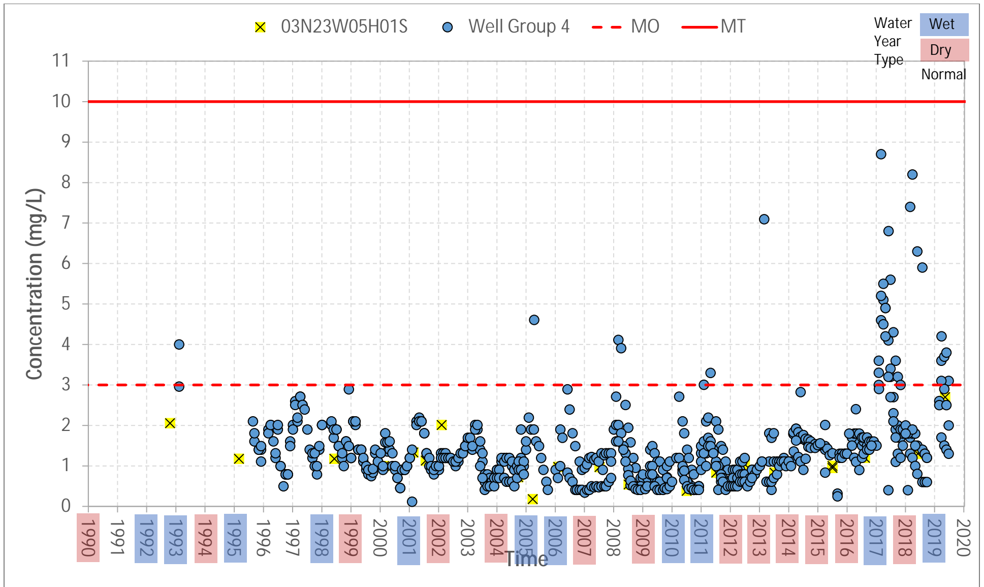
Figure I-03 Nitrate (as N) - Areas with Rising Groundwater.
