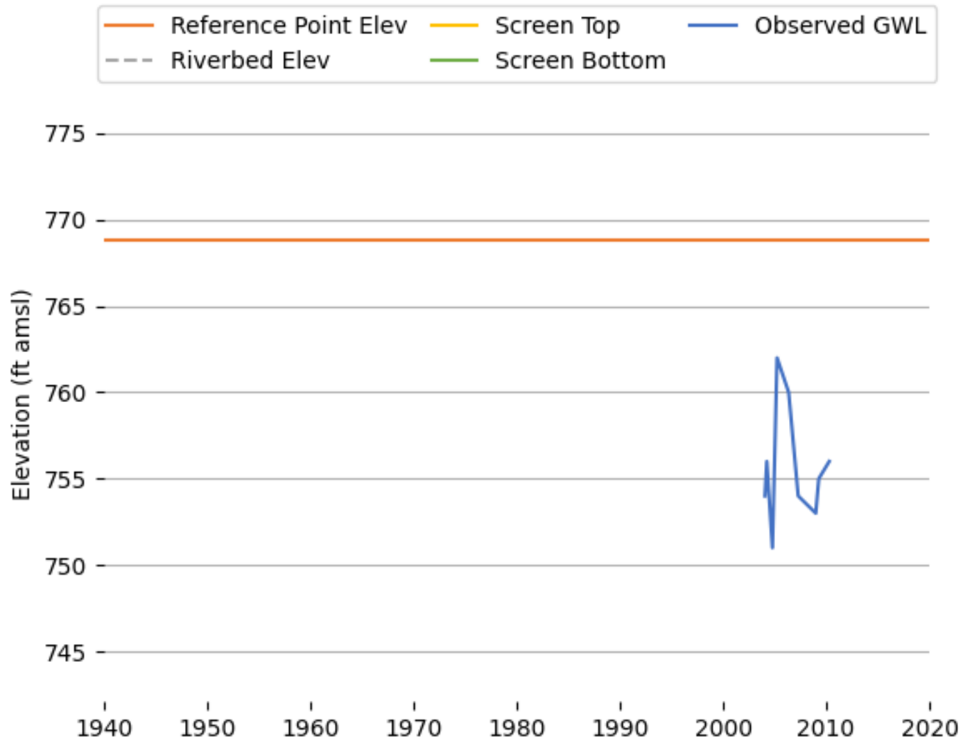
Figure K-60 Observed Groundwater Level (T0611100821_MW-7).
