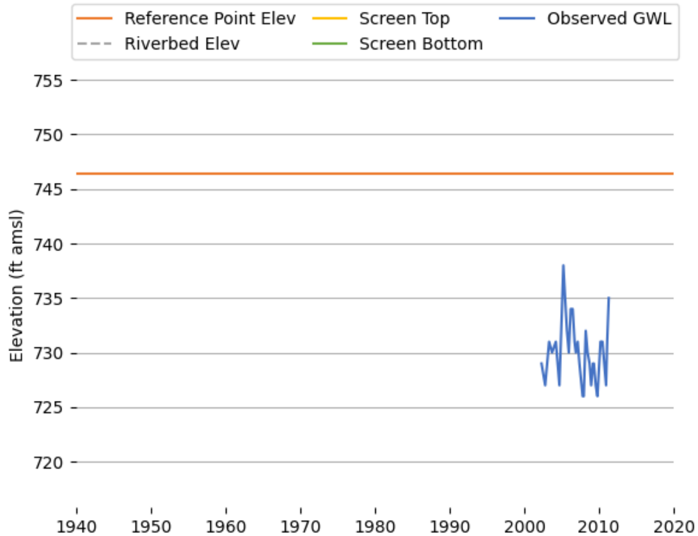
Figure K-42 Observed Groundwater Level (T0611100412_MW-14).
