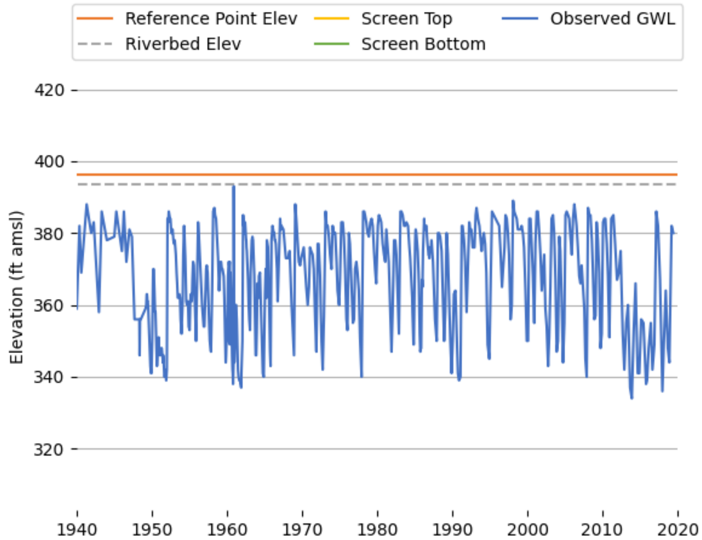
Figure K-25 Observed Groundwater Level (04N23W29F02S).
