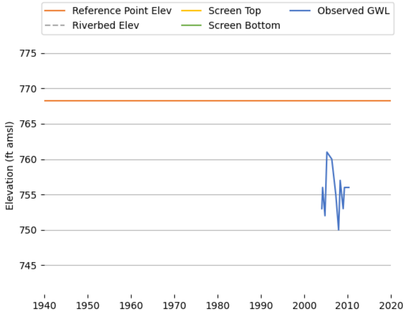
Figure K-57 Observed Groundwater Level (T0611100821_MW-4).
