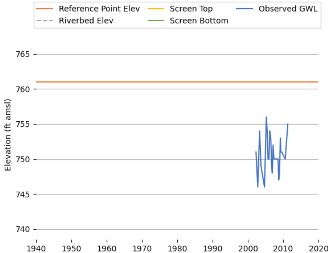
Figure K-29 Observed Groundwater Level (T0611100412_MW-1).
