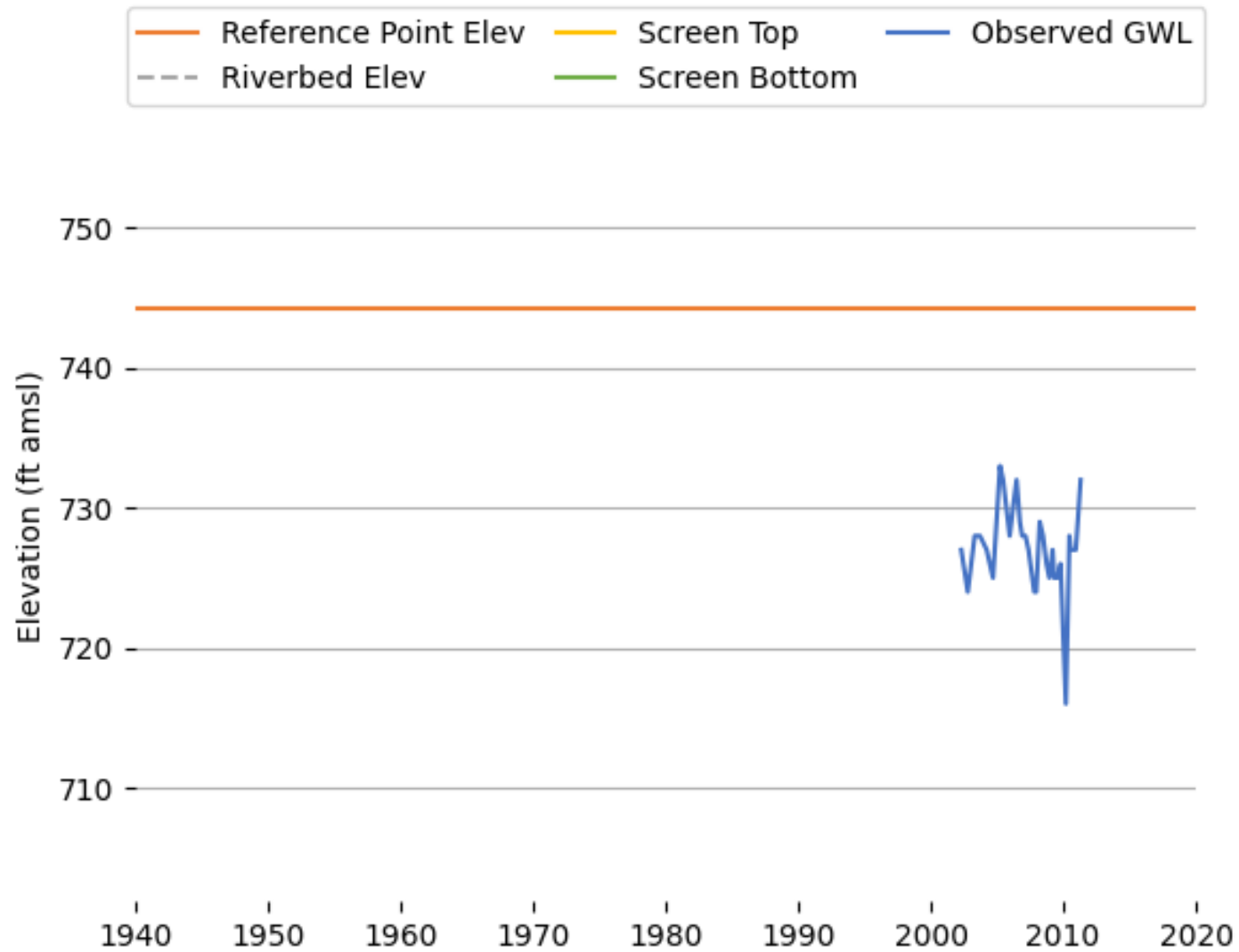
Figure K-44 Observed Groundwater Level (T0611100412_MW-16A).
