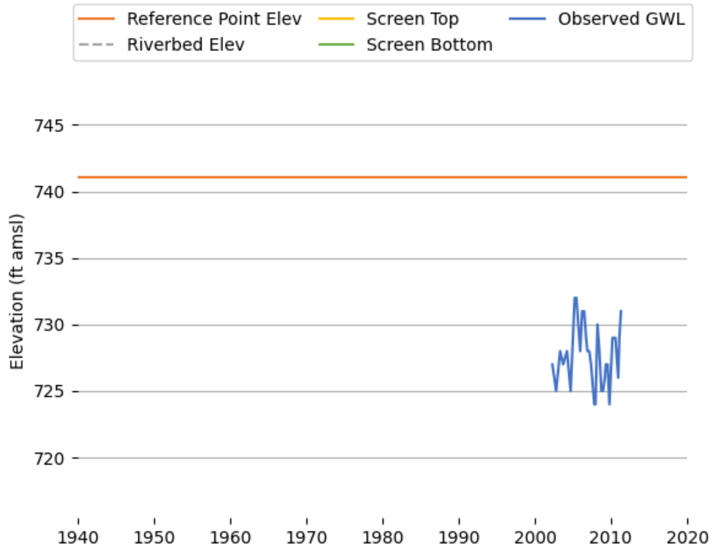
Figure K-48 Observed Groundwater Level (T0611100412_MW-20).
