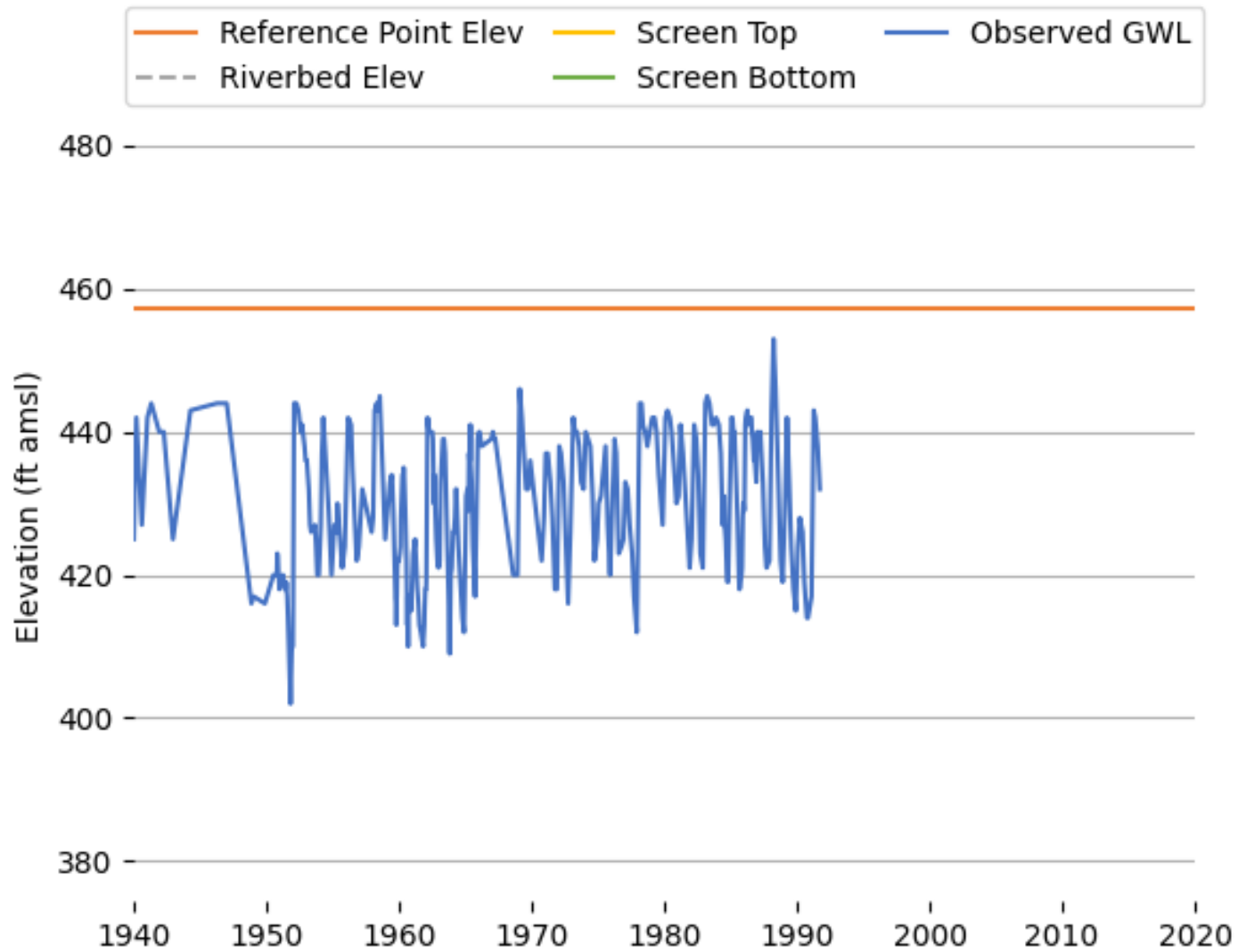
Figure K-23 Observed Groundwater Level (04N23W20J02S).
