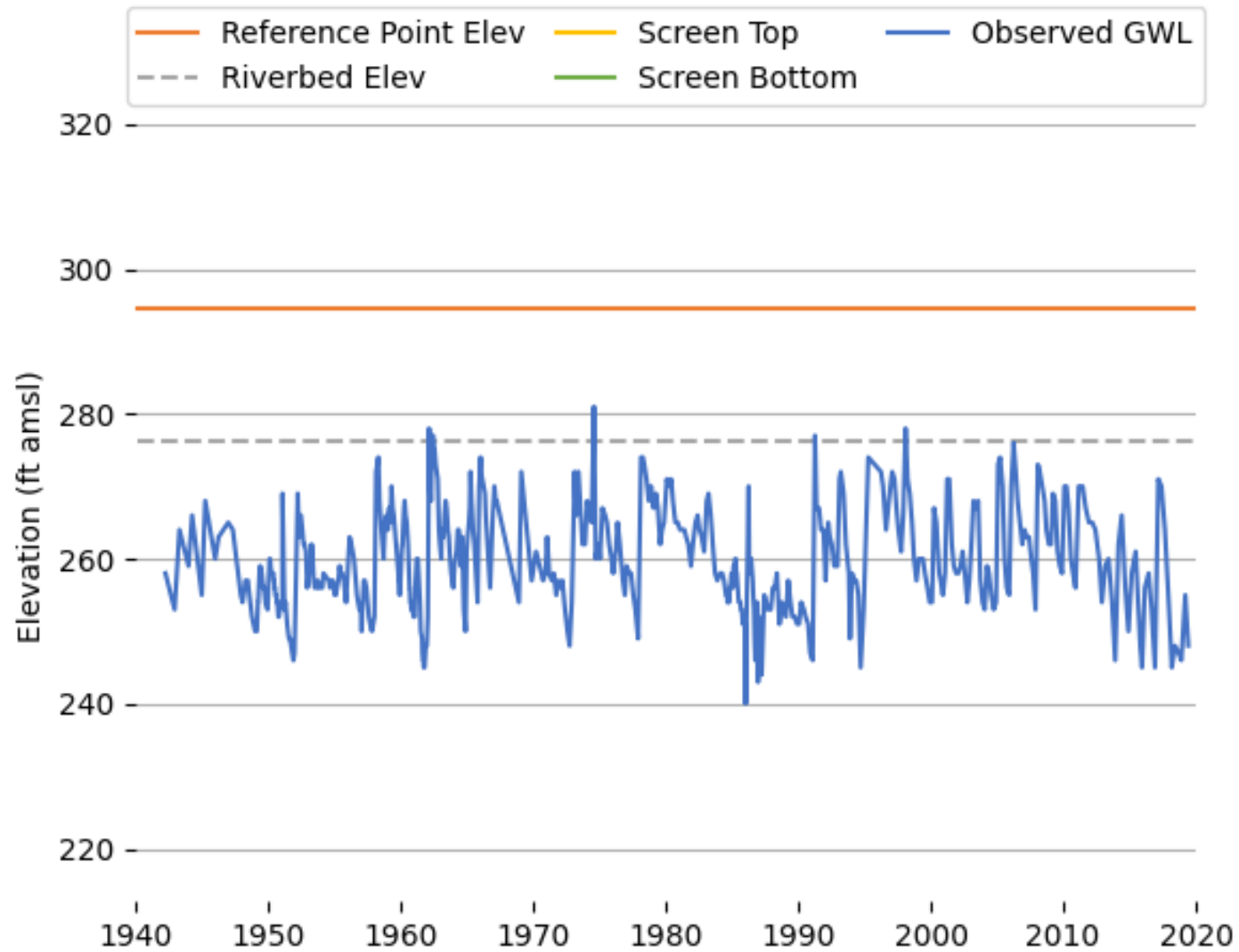
Figure K-03 Observed Groundwater Level (03N23W05B01S).
