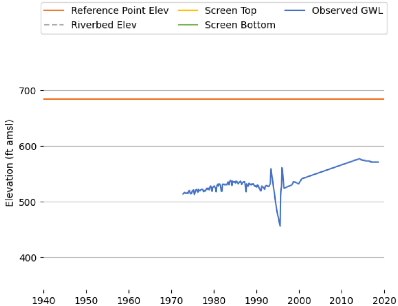
Figure K-15 Observed Groundwater Level (04N23W15B01S).
