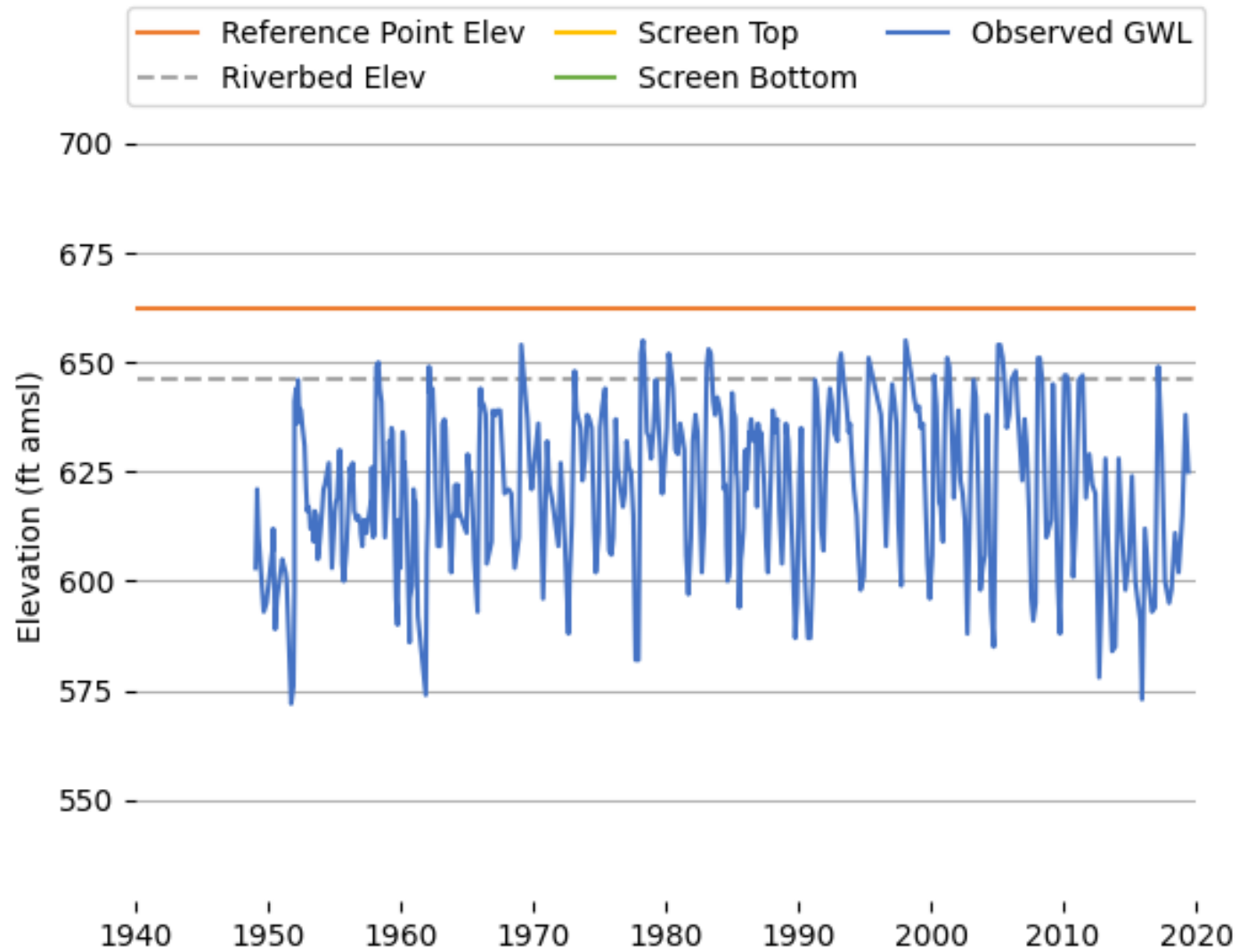
Figure K-11 Observed Groundwater Level (04N23W09B01S).
