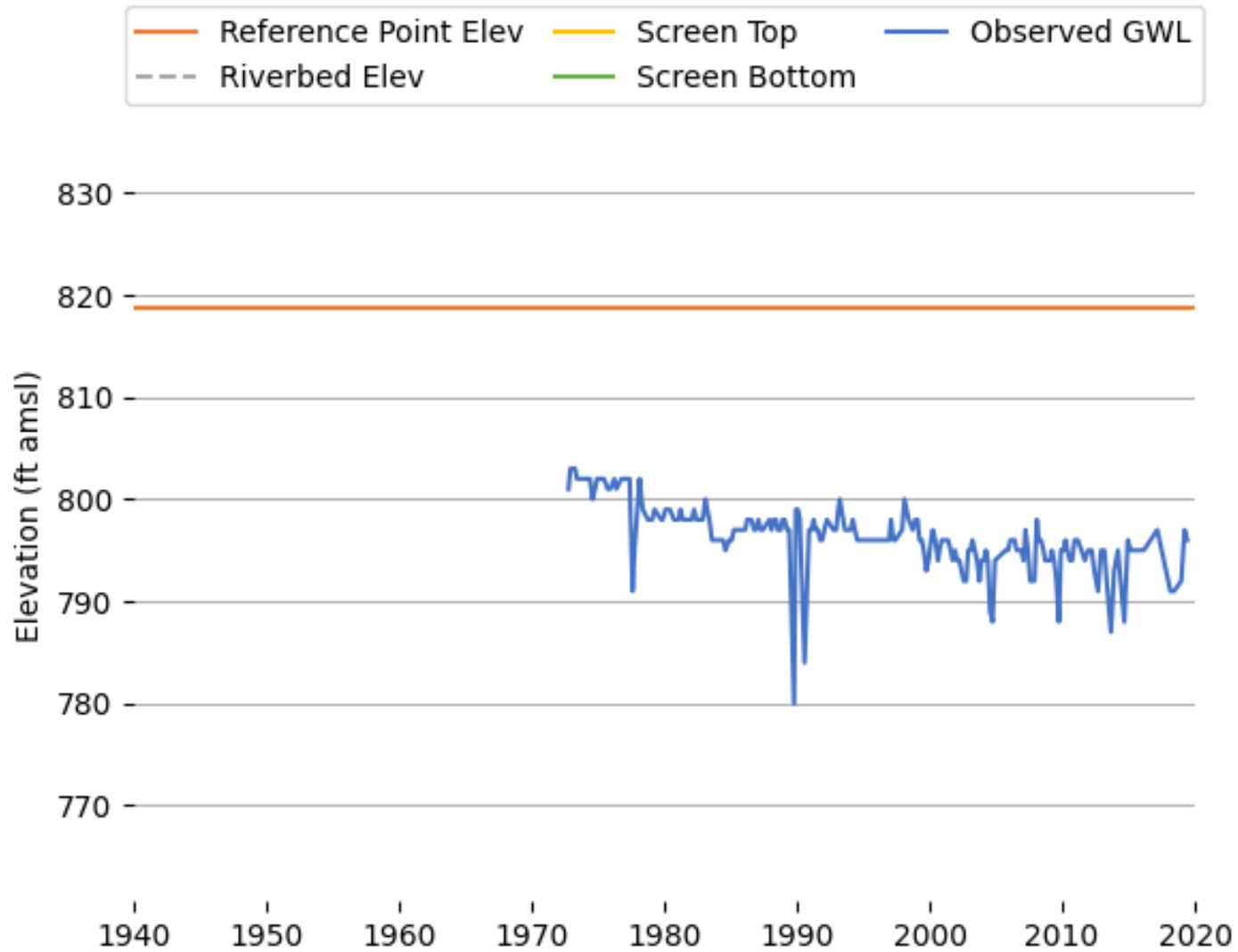
Figure K-28 Observed Groundwater Level (05N23W33G01S).
