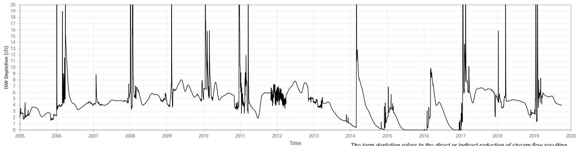
Figure N-08 Streamflow Depletion (Subsurface Dam).
