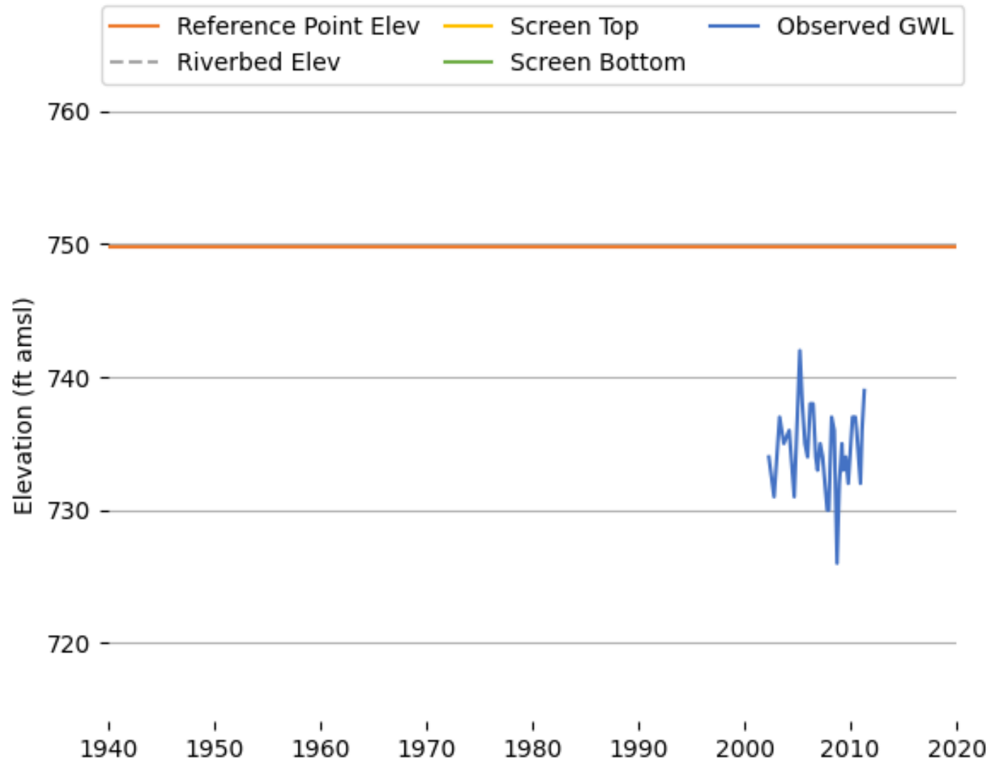
Figure K-41 Observed Groundwater Level (T0611100412_MW-13).
