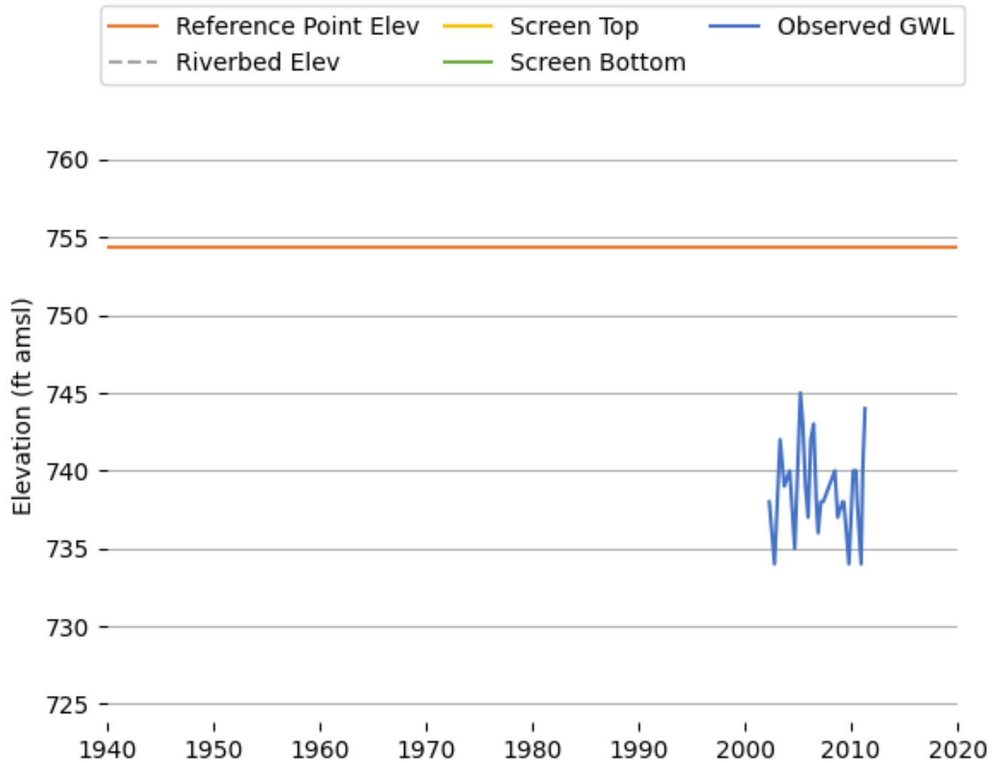
Figure K-39 Observed Groundwater Level (T0611100412_MW-11).
