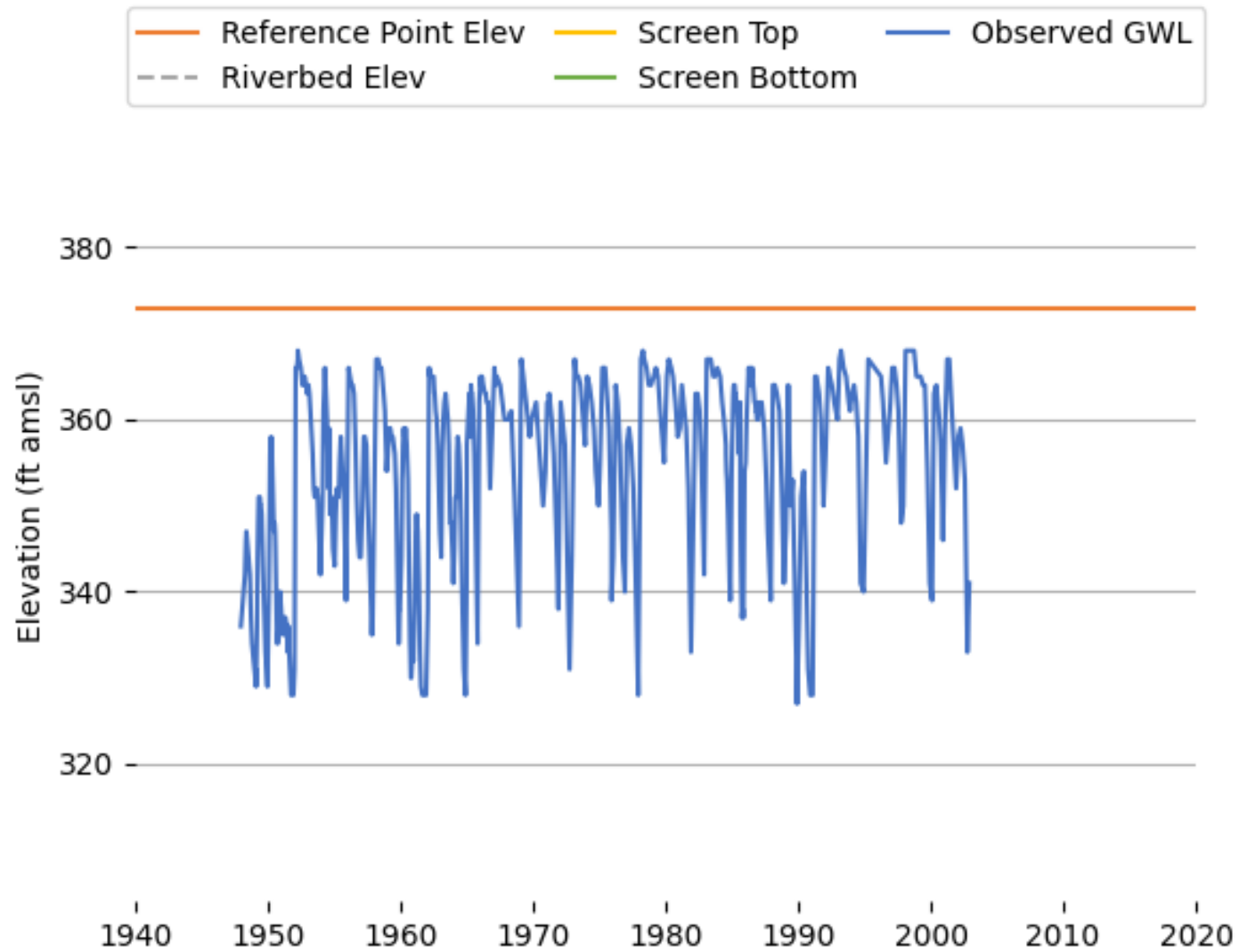
Figure K-26 Observed Groundwater Level (04N23W29L01S).
