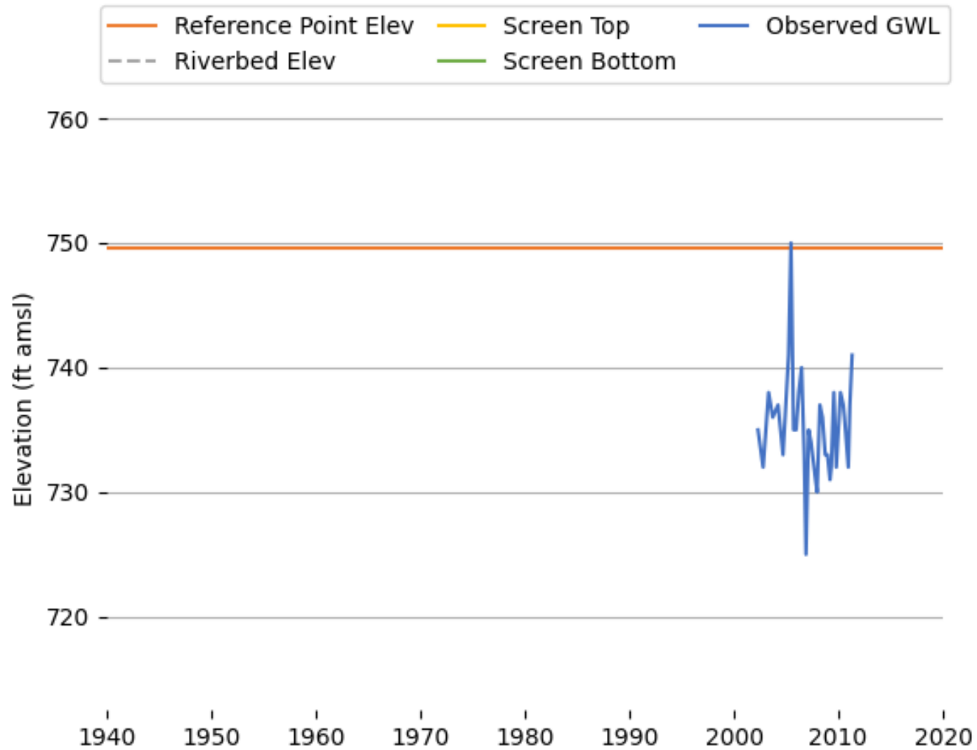
Figure K-35 Observed Groundwater Level (T0611100412_MW-7).
