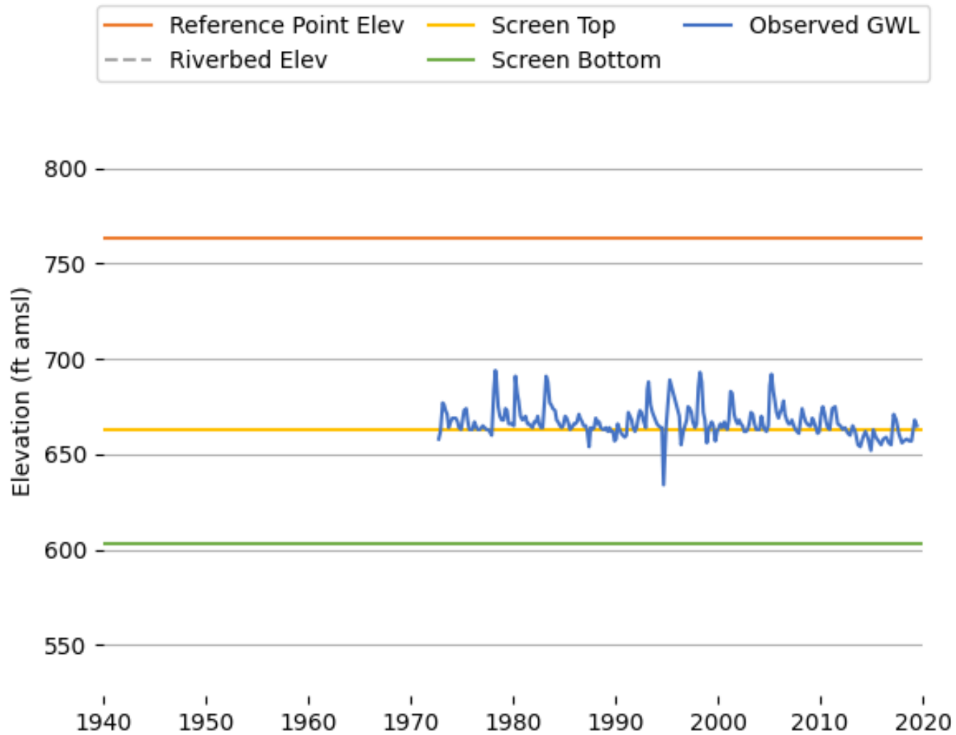
Figure K-09 Observed Groundwater Level (04N23W03M01S).
