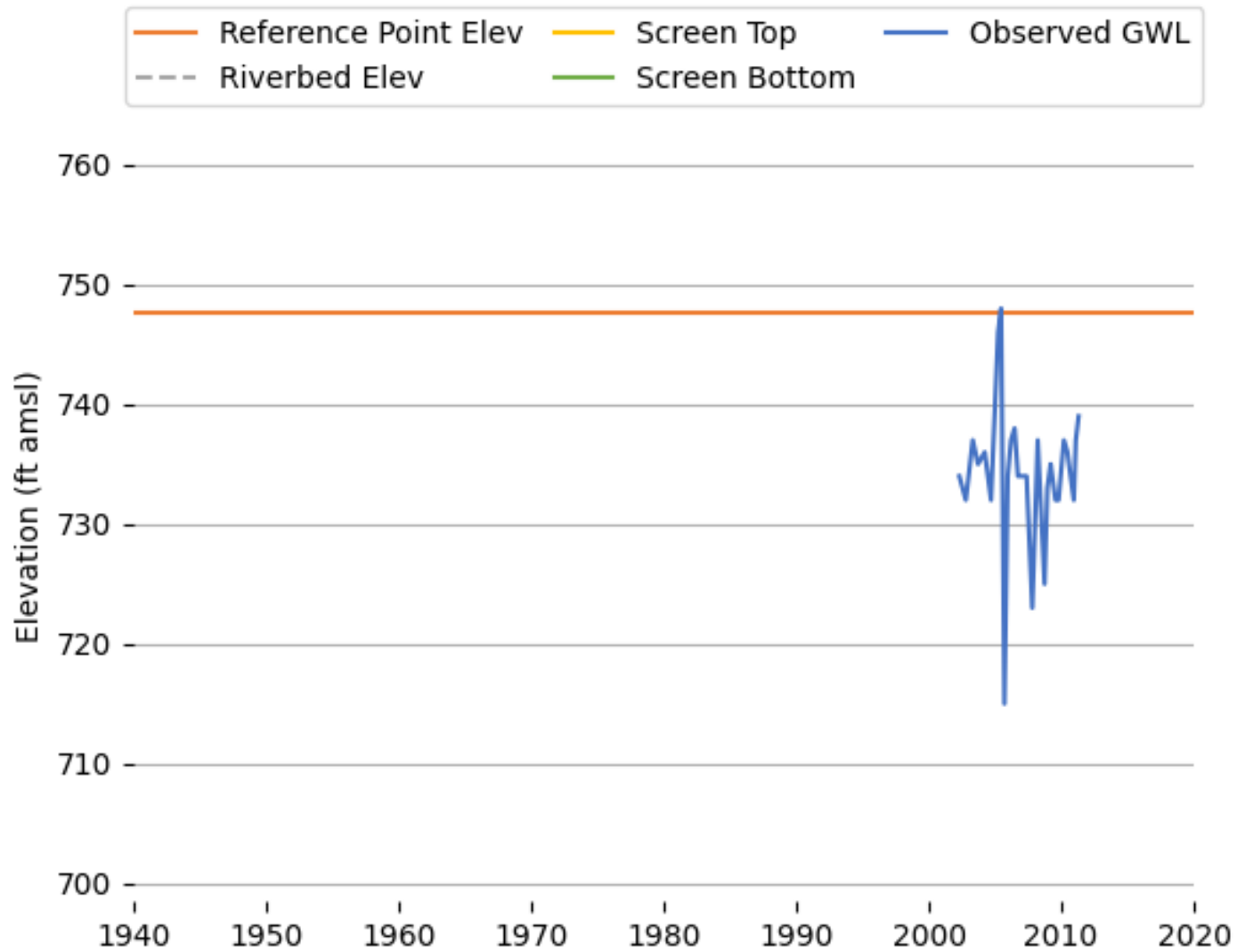
Figure K-36 Observed Groundwater Level (T0611100412_MW-8).
