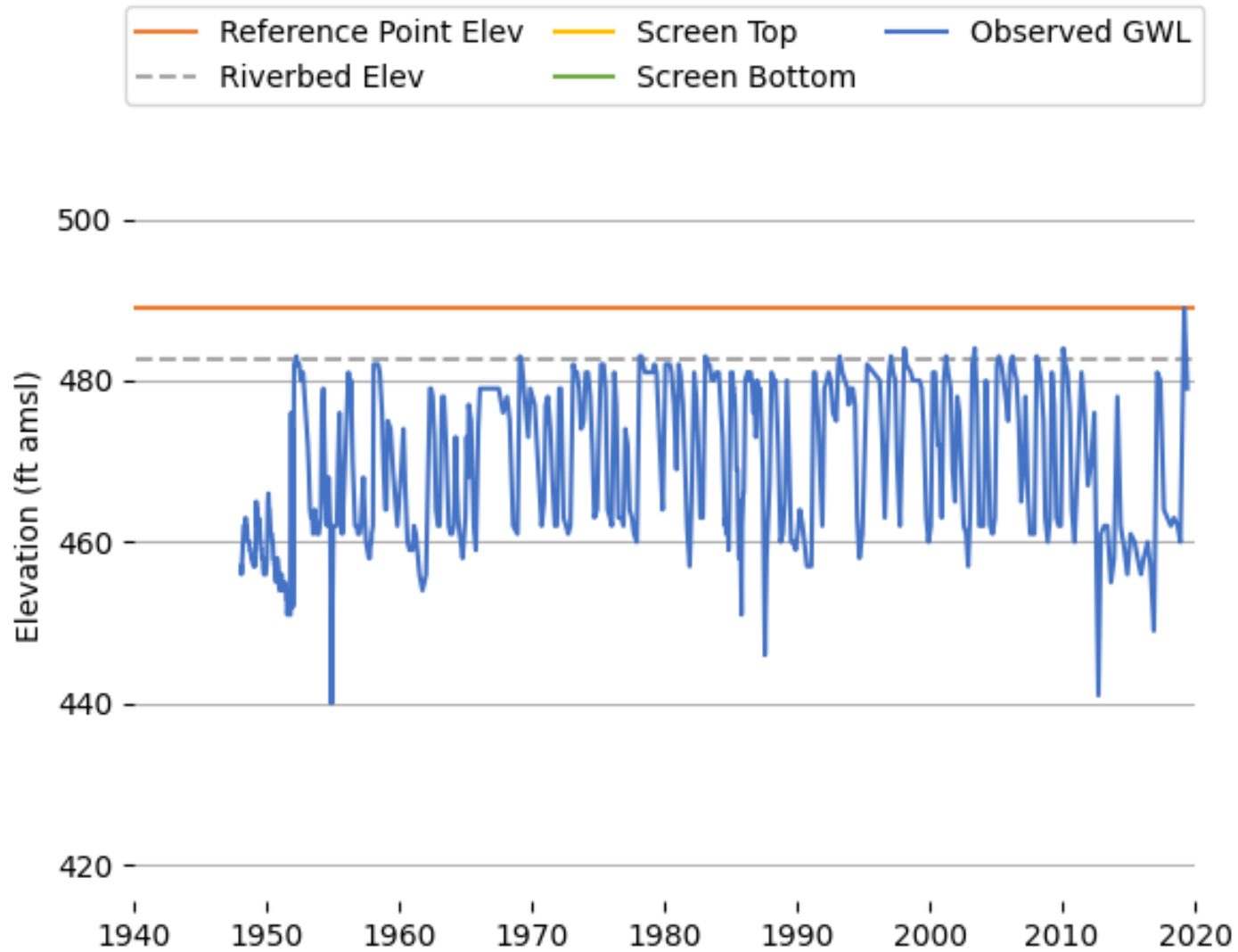
Figure K-21 Observed Groundwater Level (04N23W20A01S).
