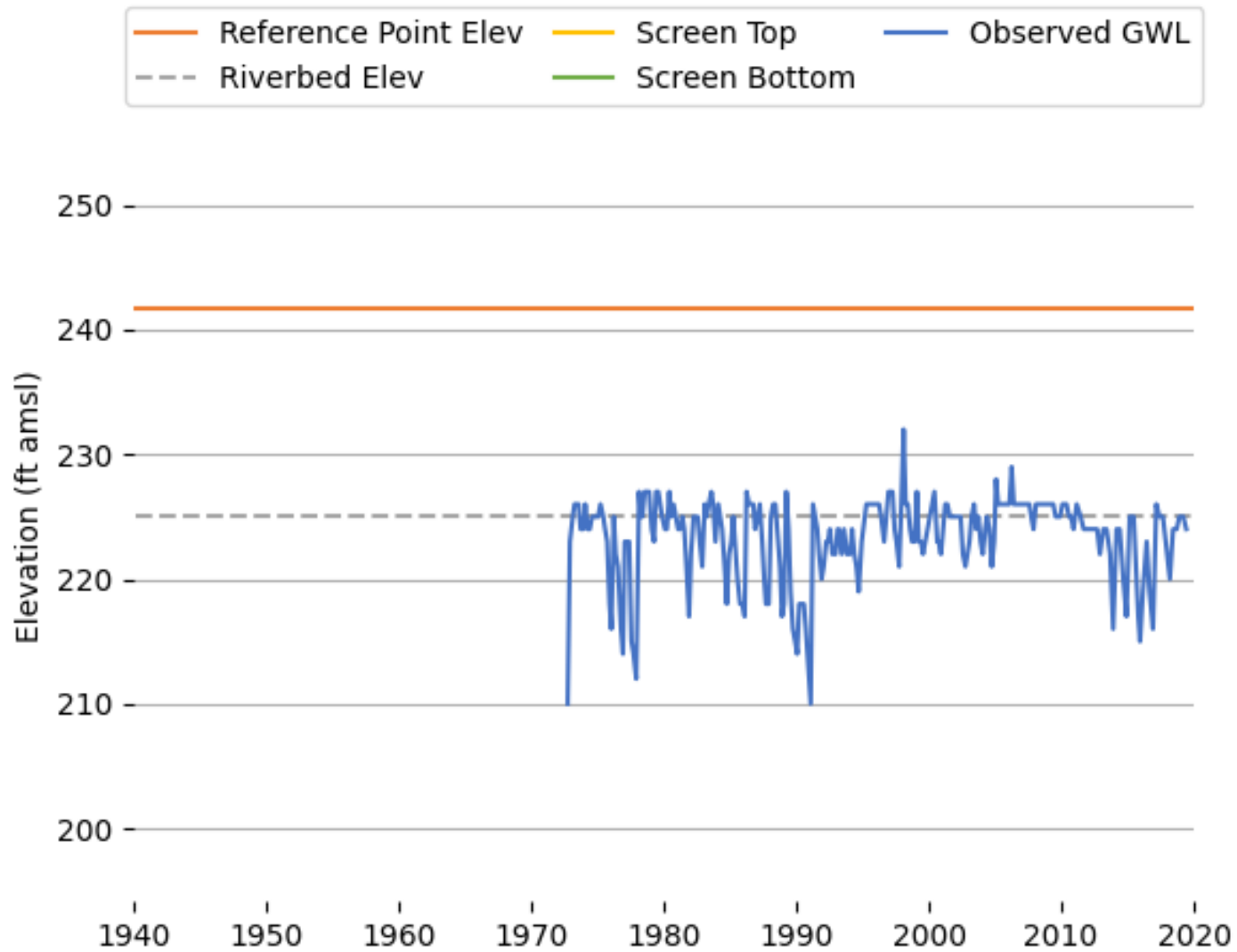
Figure K-06 Observed Groundwater Level (03N23W08B07S).
